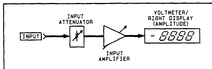
DC Level Measurement Block Diagram
