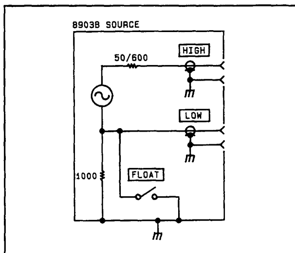
Simplified Schematic of the Audio Analyzer Source Output
