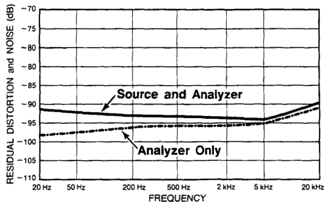
Figure 1-2. Typical Combined Source and Analyzer Residual Distortion With V_{source} Set to 1.5V (80 kHz BW)
