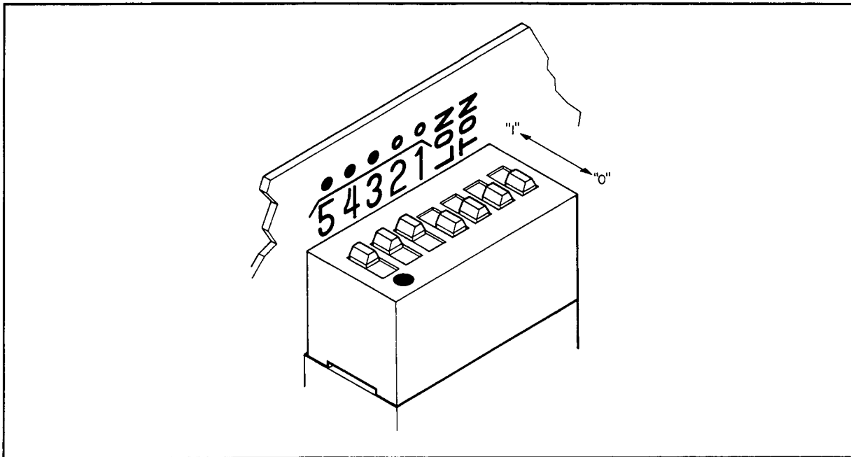
Figure 2-3. HP-IB Address Switch Shown as Set by the Factory. The Address Shown is 11100 in Binary with Both Talk Only and Listen Only Off.
