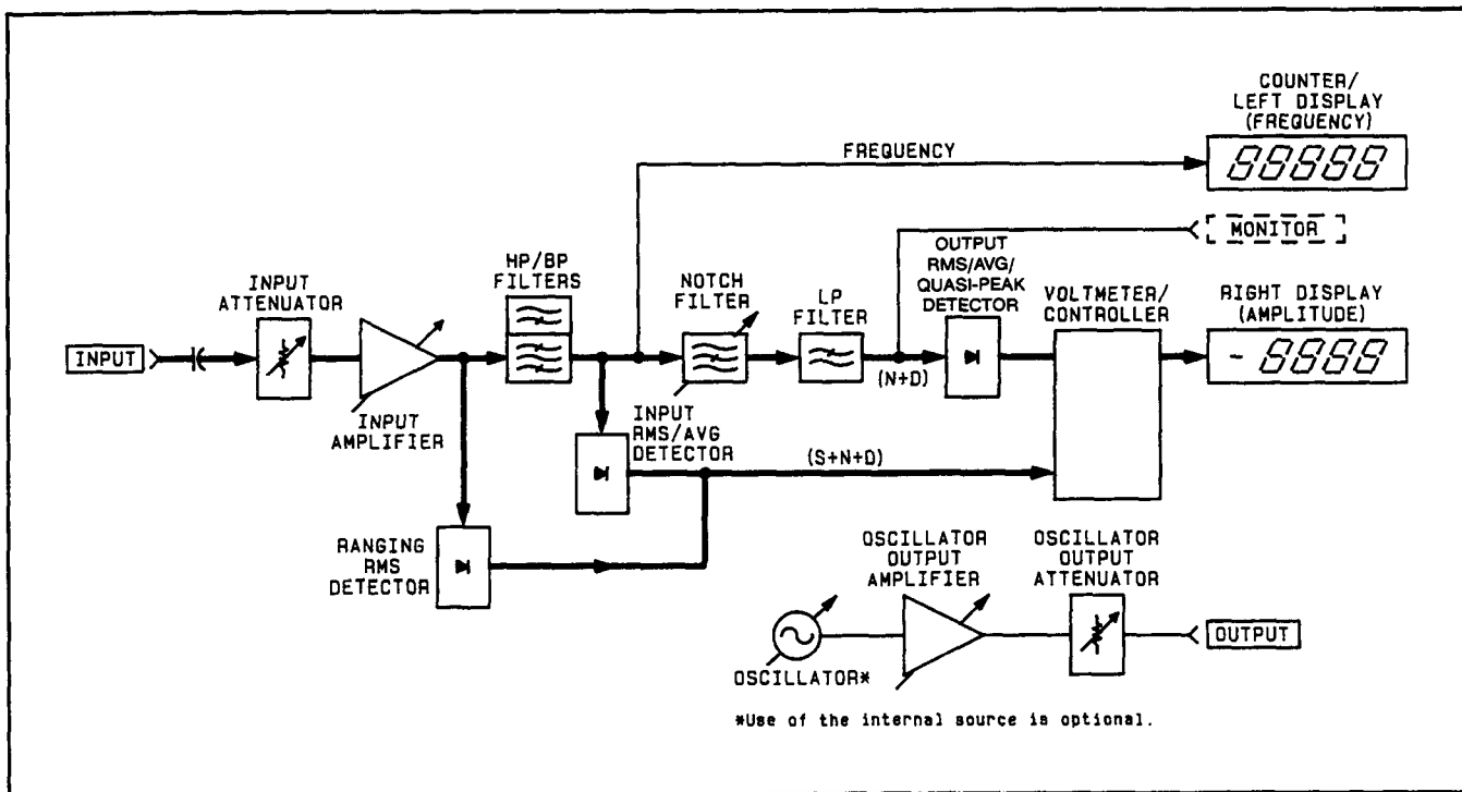
Distortion Measurement Block Diagram
