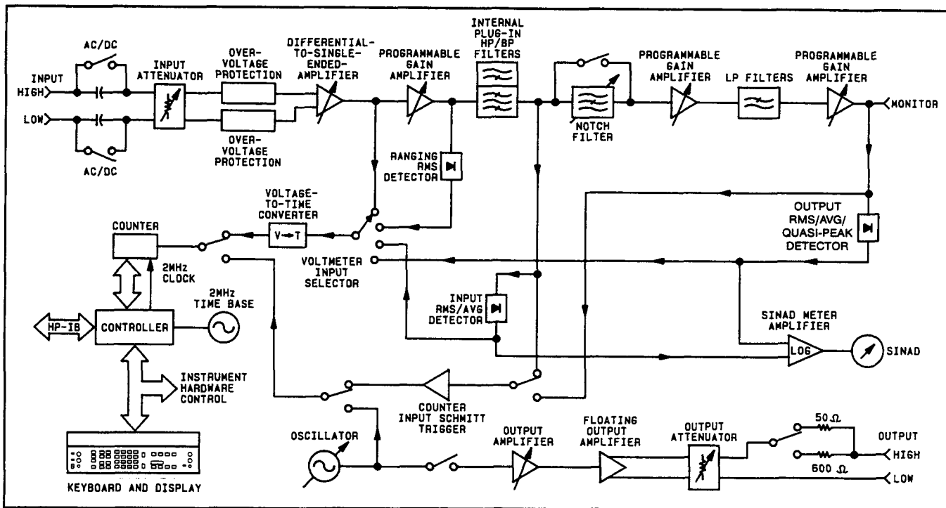
Figure 1-5. Simplified HP 8903B Audio Analyzer Block Diagram
