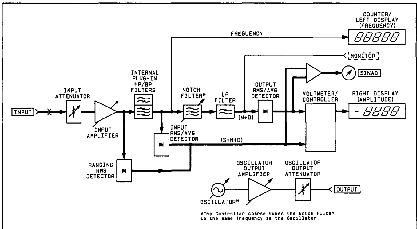
SINAD Measurement Block Diagram
