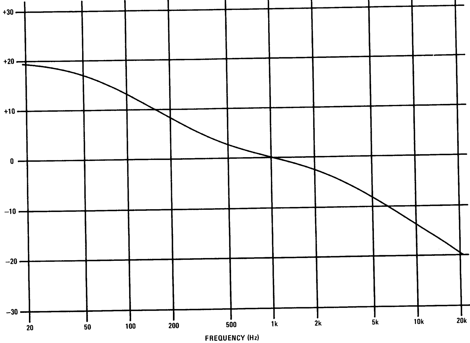
Theoretical RIAA Response Curve
