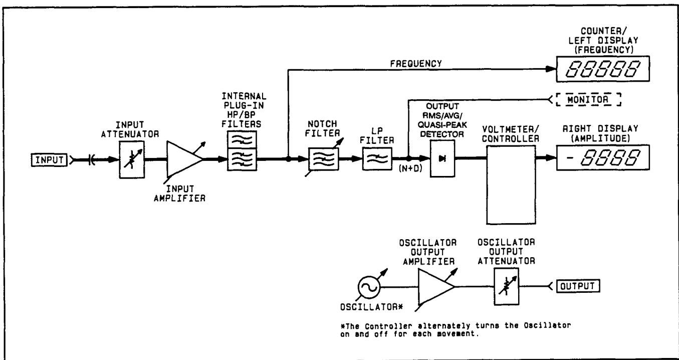
Signal-To-Noise Measurement Block Diagram
