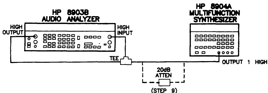
Figure 4-1. Distortion, SINAD, and Signal-to-Noise Accuracy Test Setup
