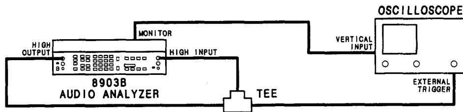
Figure 5-3. Notch Filter Tune and Balance Adjustment Test Setup
