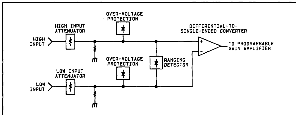
Analyzer Input Block Diagram
