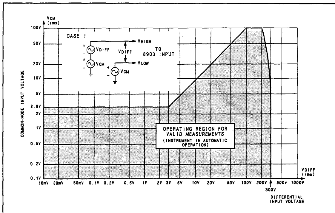
CASE 1. Single-Ended Source with Common Mode on Both Lines
