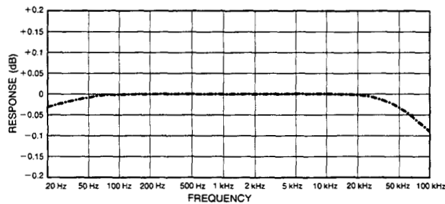
Figure 1-1. Typical Combined Source and AC Level Flatness
