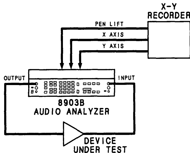
X-Y Recording Setup
