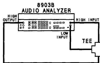
Figure 5-2. Common-Mode Rejection Adjustment Test Setup
