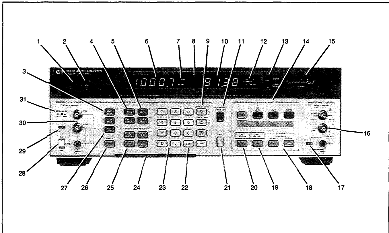
Figure 3-1. Front-Panel Features
