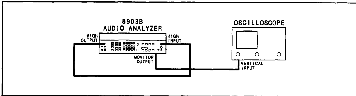
Figure 3-3. Basic Functional Checks Setup
