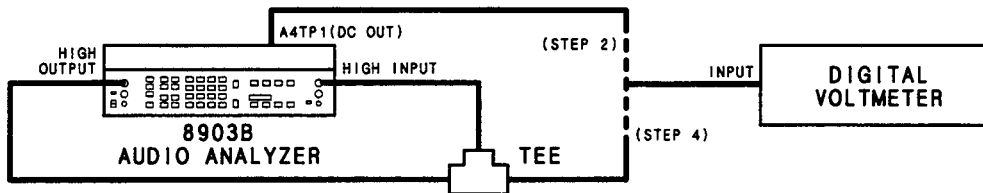
Figure 5-4. Voltmeter Adjustment Test Setup
