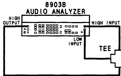
Figure 4-2. Common-Mode Rejection Ratio Test Setup
